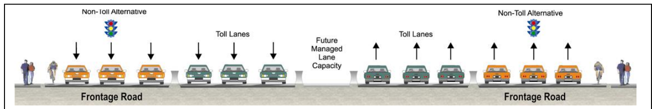
Figure 11 Typical Toll Road Cross Section (TOLL FWY 6)
