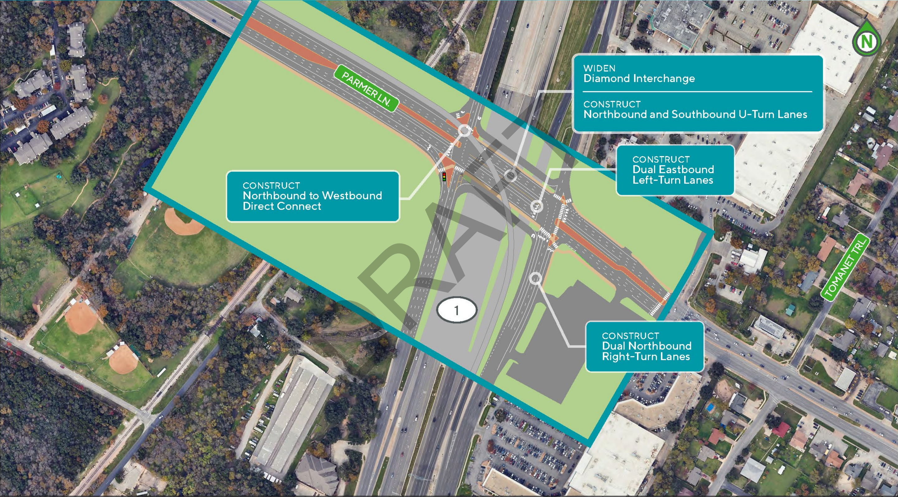
Figure 15: Long-Term Intersection Improvements: Loop 1 / FM 734
