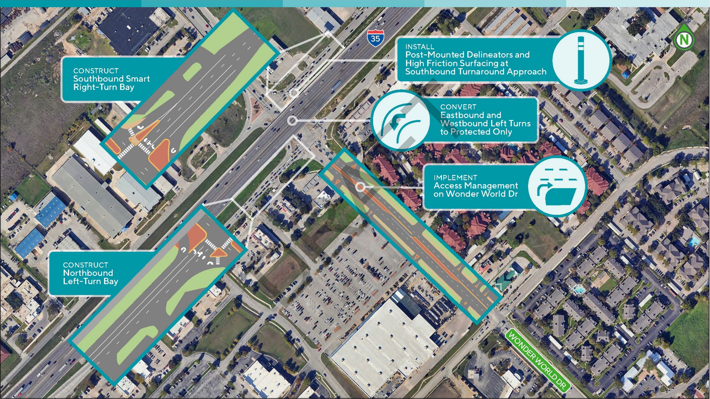
Figure 10: Near-Term Intersection Improvements: IH-35 / RM 12
