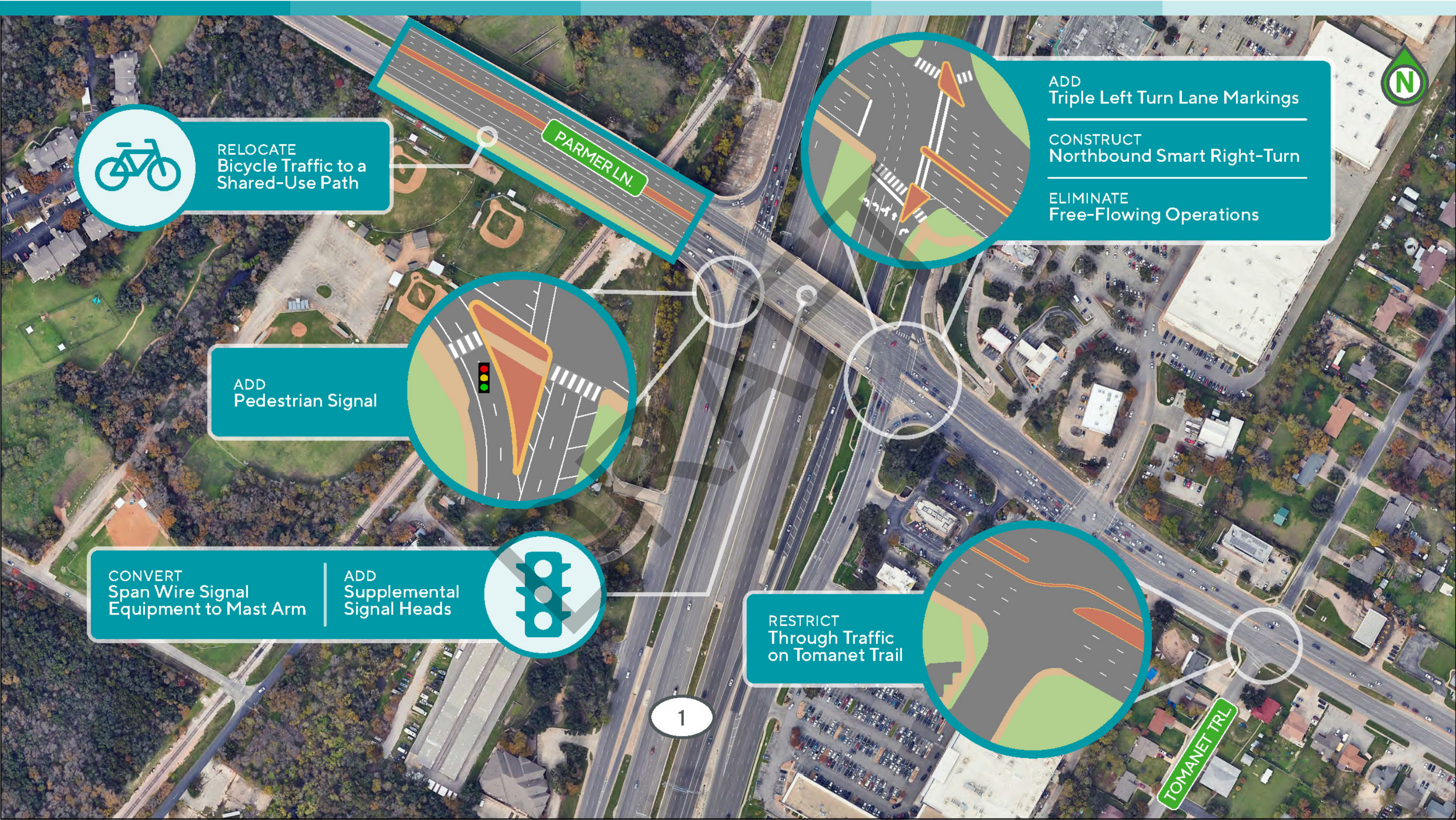
Figure 12: Near-Term Intersection Improvements: Loop 1 / FM 734
