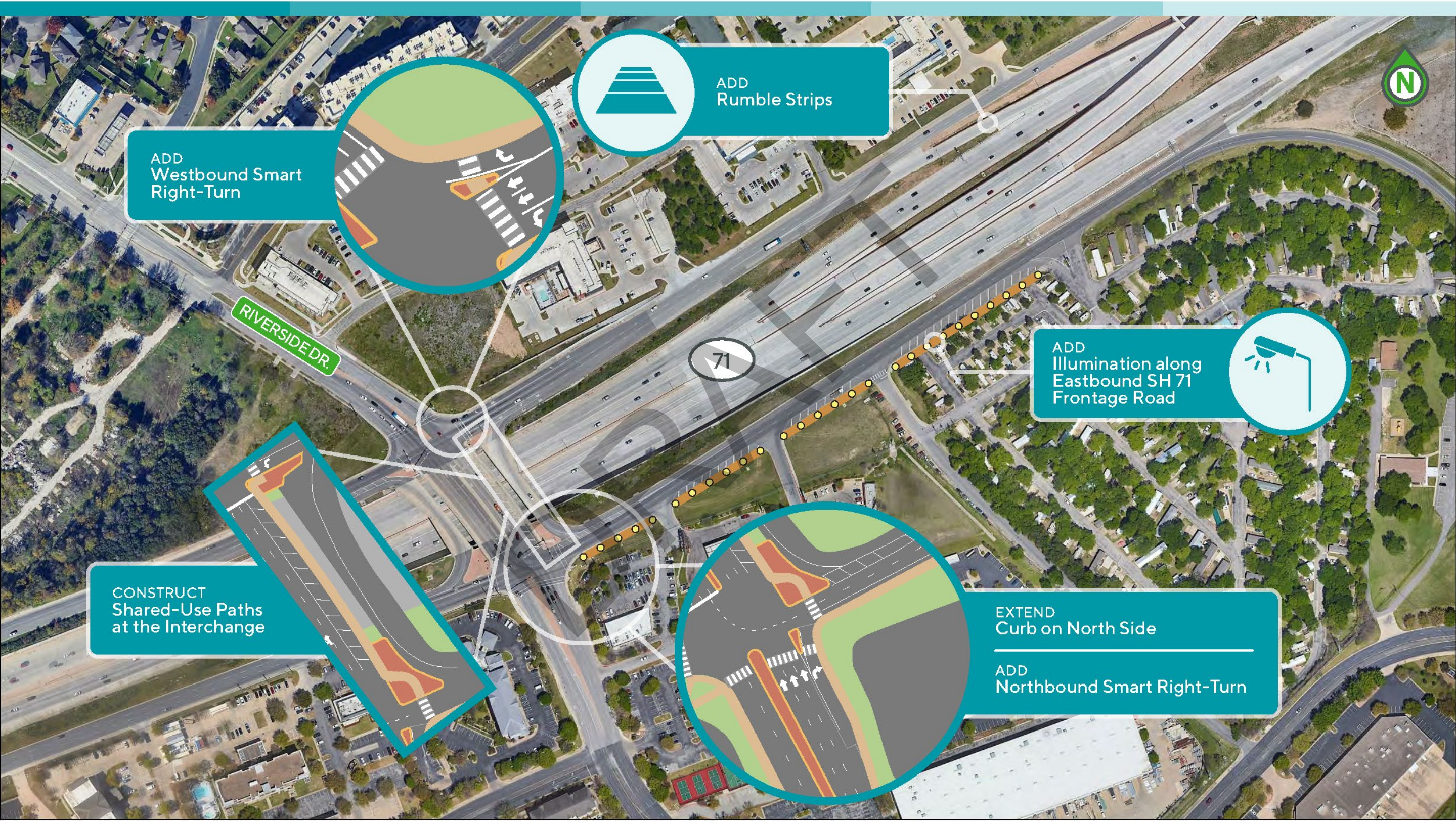
Figure 9: Near-Term Intersection Improvements: SH 71 / Riverside Drive
