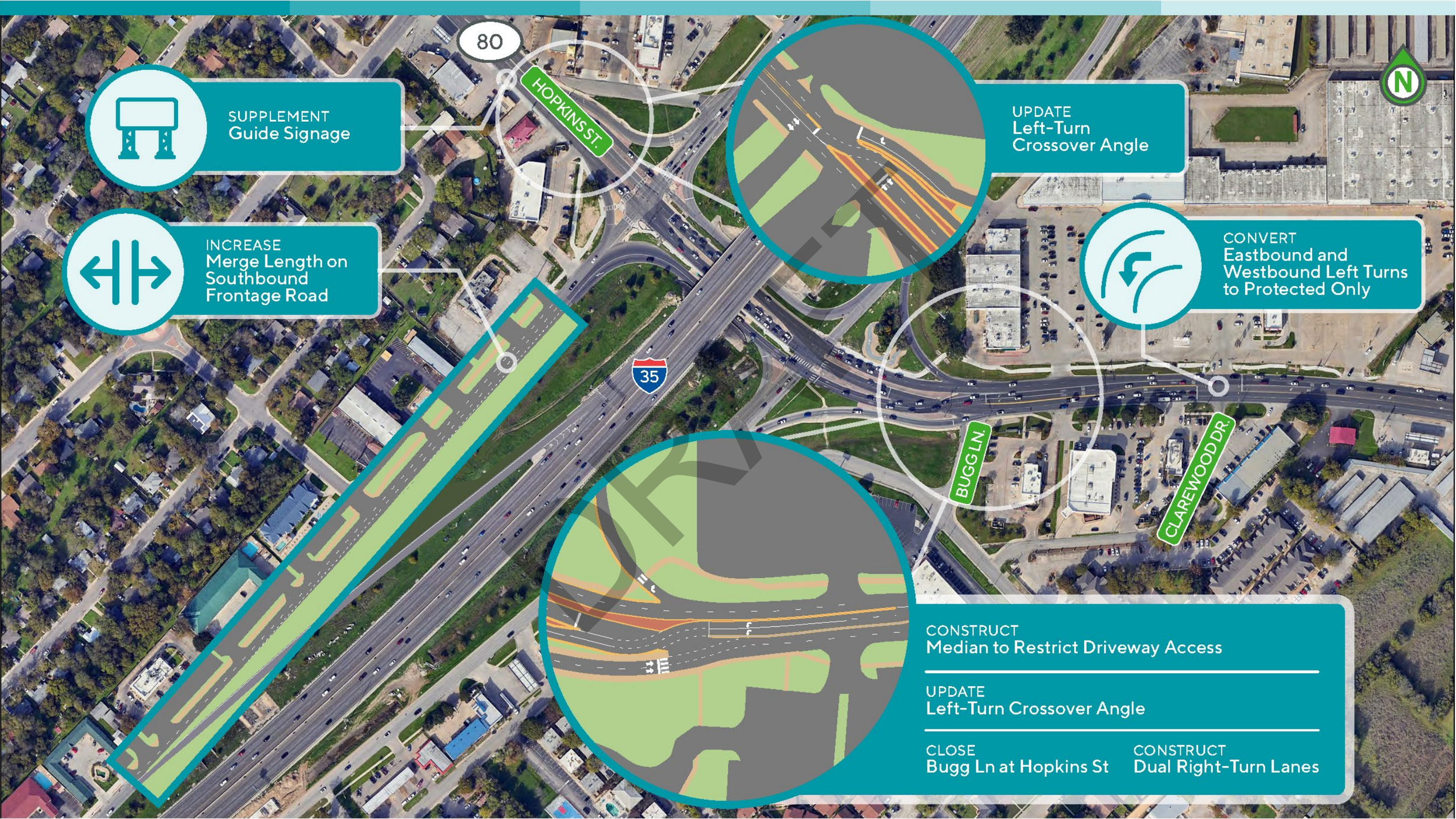
Figure 11: Near-Term Intersection Improvements: IH-35 / SH 80
