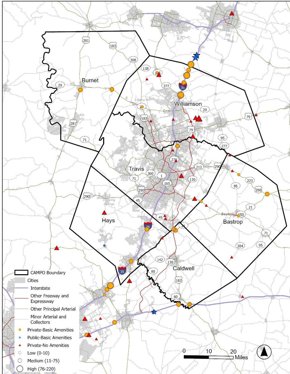
Figure 1: CAMPO Region Truck Parking Facilities
